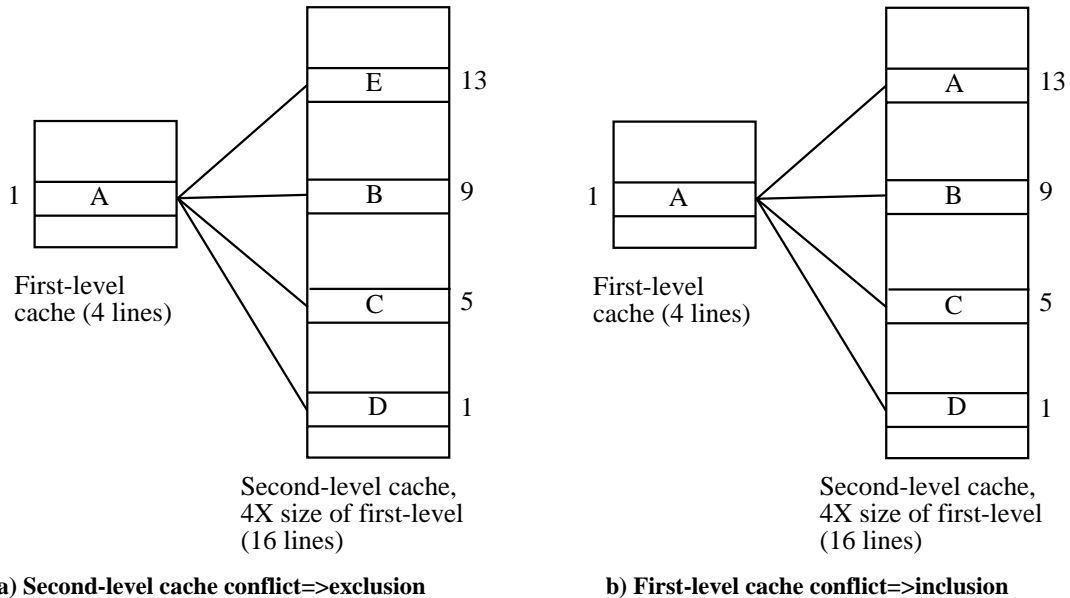
Figure 21: Exclusion vs. inclusion during swapping, direct-mapped caches
