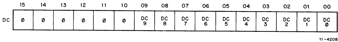
Figure 7-10 Desired Cylinder Register
