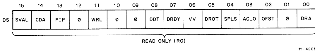
Figure 7-7 Drive Status Register
