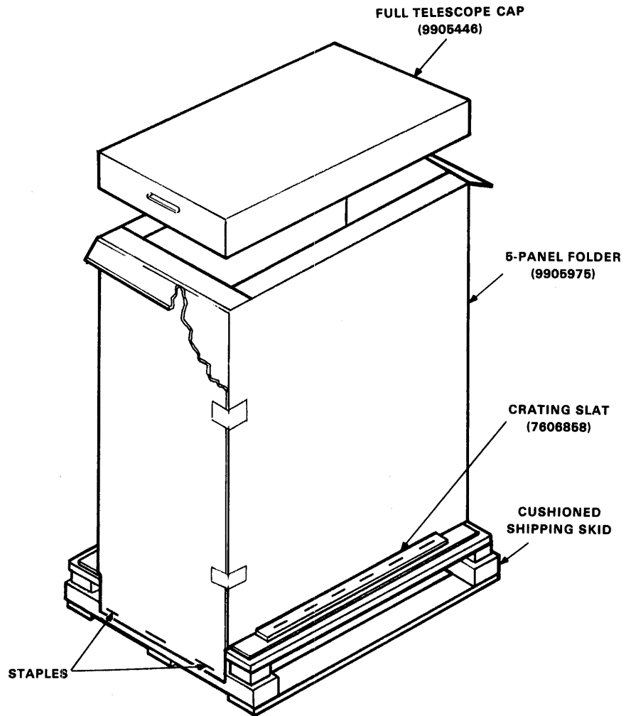
Figure 4-1 RK06/RK07 Shipping Package Configuration
