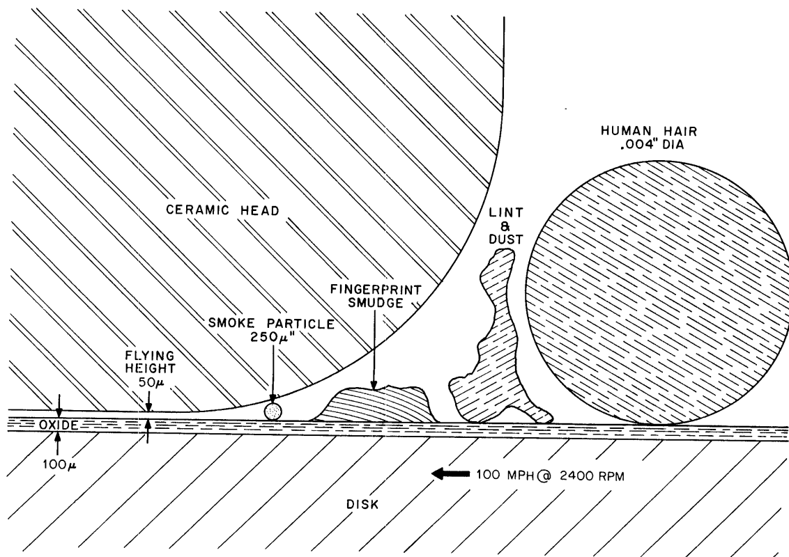
Figure 3-1 Relationship of Disk Head, Disk, and Contaminants
