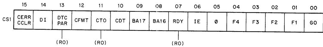
Figure 7-2 Control/Status Register 1
