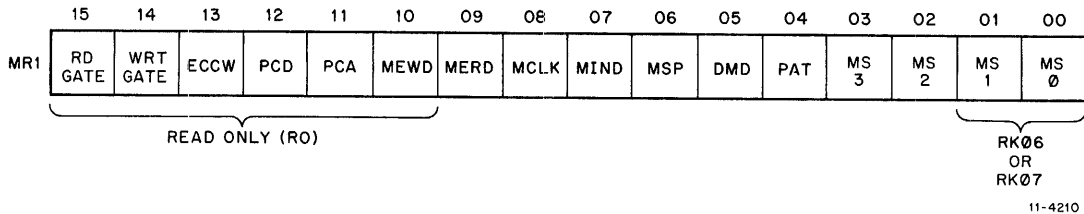
Figure 7-12 Maintenance Register 1
