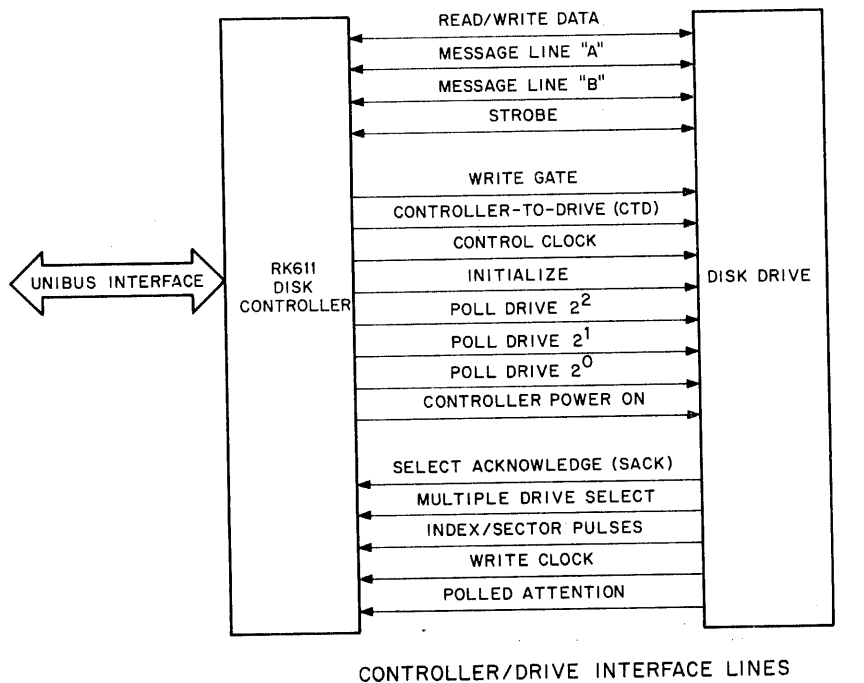
Figure 2-6 Interface Lines
