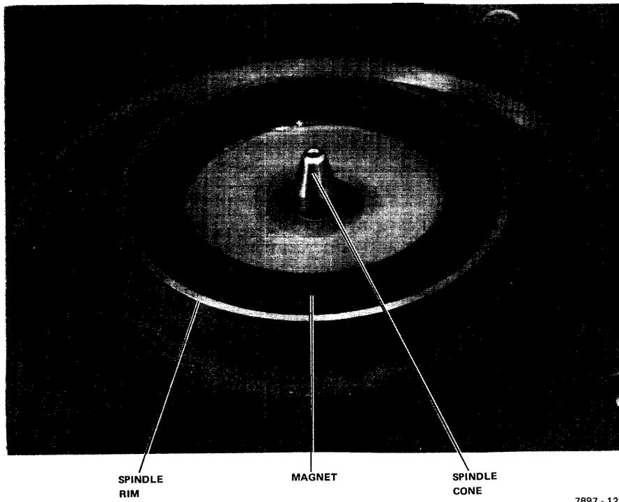
Figure 8-1 Spindle Assembly
