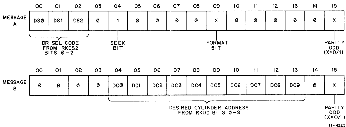
Figure 7-27 Seek Command
