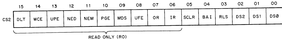
Figure 7-6 Control/Status Register 2
