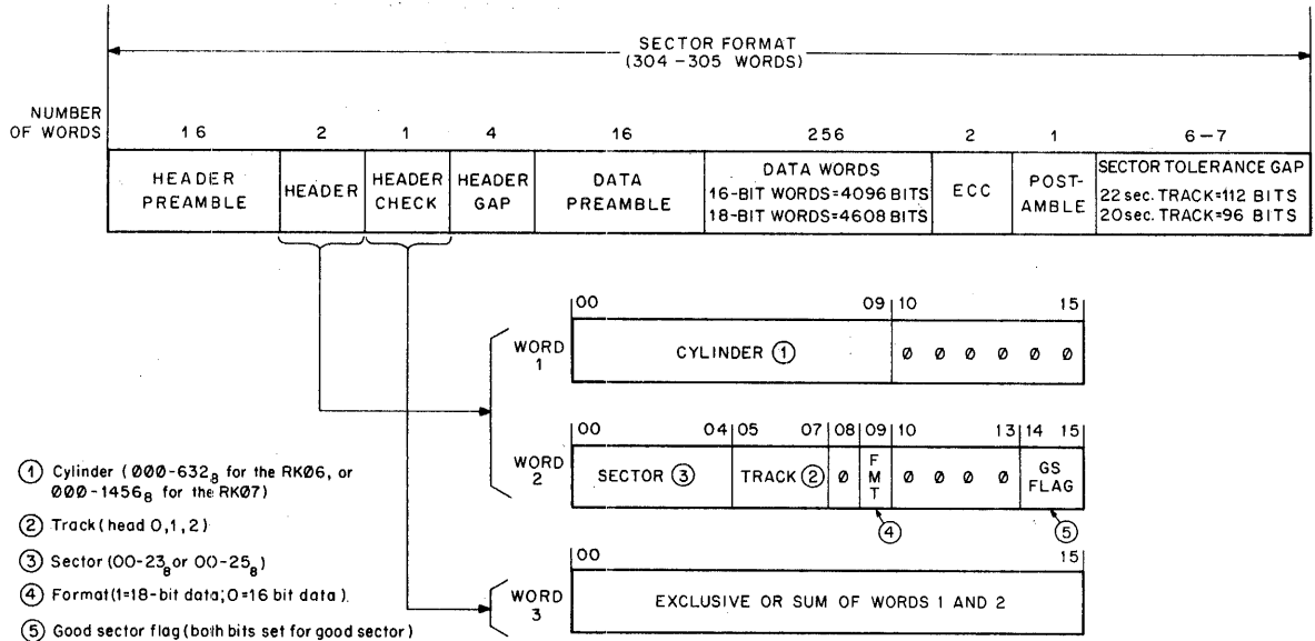
Figure 2-3 Sector Formats
