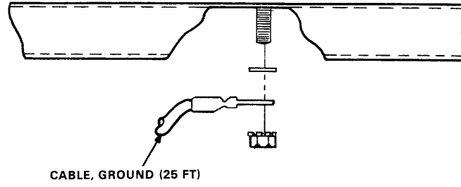
VIEW C-C
