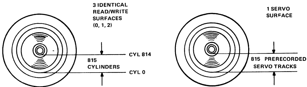
SERVO SURFACE (TIMING & POSITION)
