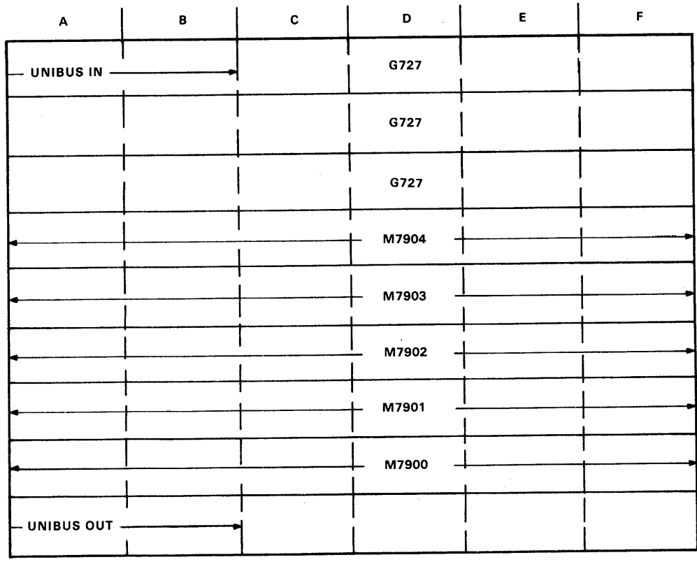
Figure 4-4 RK611 Controller Backplane (from Module Side)
