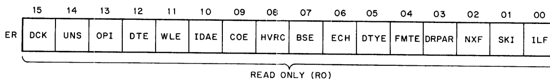
Figure 7-8 Drive Error Register
