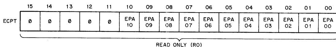
Figure 7-14 ECC Pattern Register
