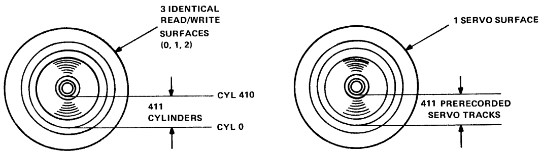
SERVO SURFACE (TIMING & POSITION)
