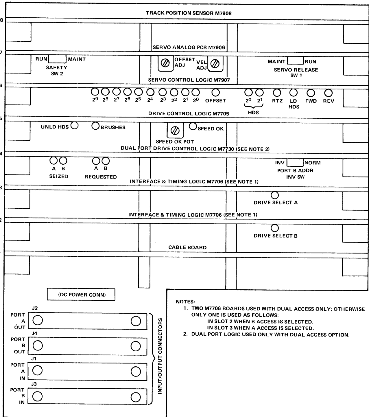
Figure 4-3 RK07 Disk Drive Logic Module Locations
