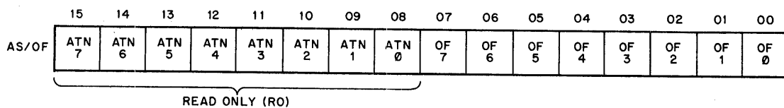
Figure 7-9 Attention Summary/Offset Register
