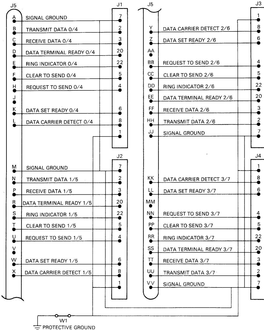
Figure 2-7 H3173-A Circuit Diagram
