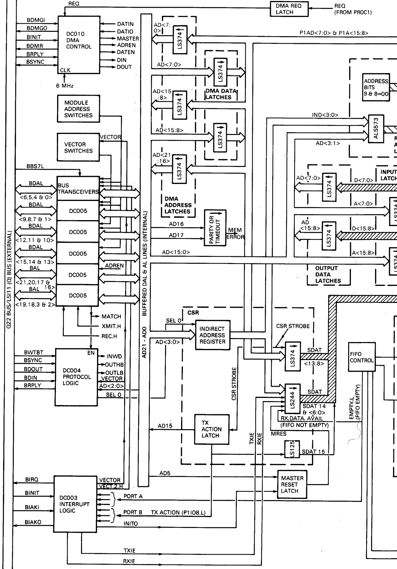
Figure 4-1 DHV11 Block Diagram
