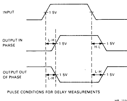
Figure A-17 DC010 Voltage Waveforms
