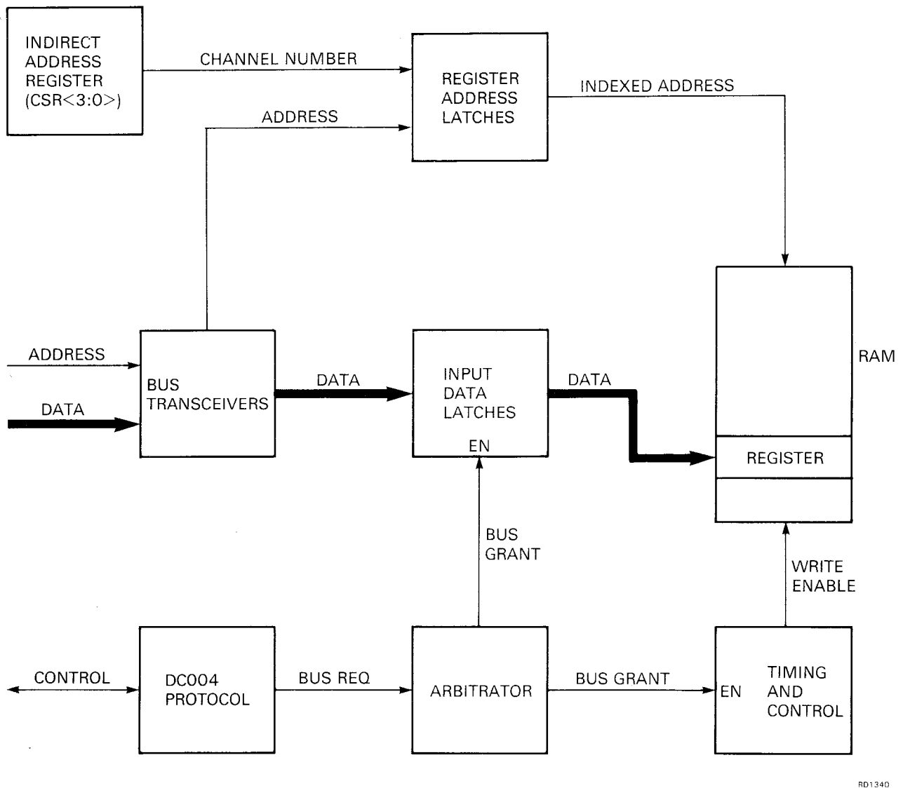
Figure 4-9 Writing to a Register
