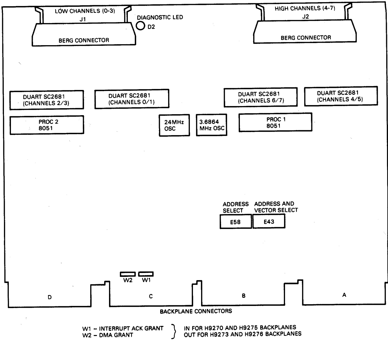
Figure 1-1 M3104 Module
