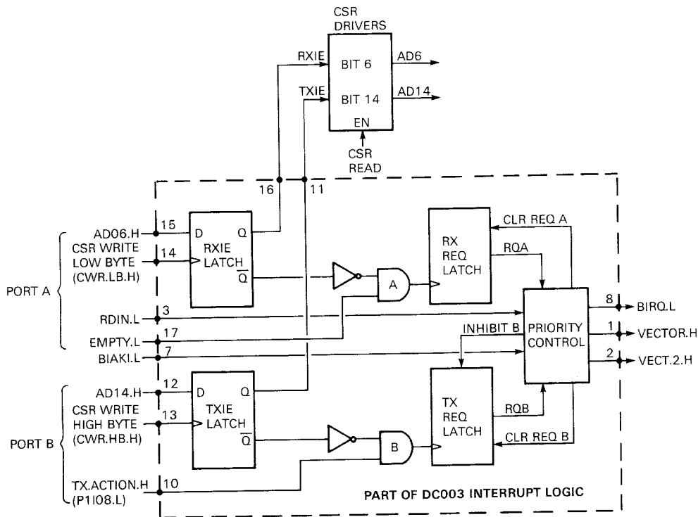
Figure 4-17 Interrupt Logic
