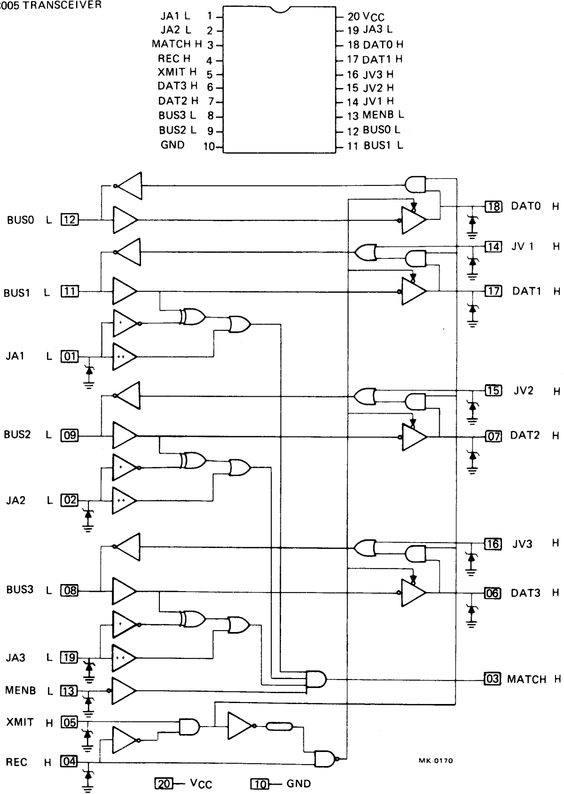
Figure A-13 DC005 Simplified Logic Diagram
