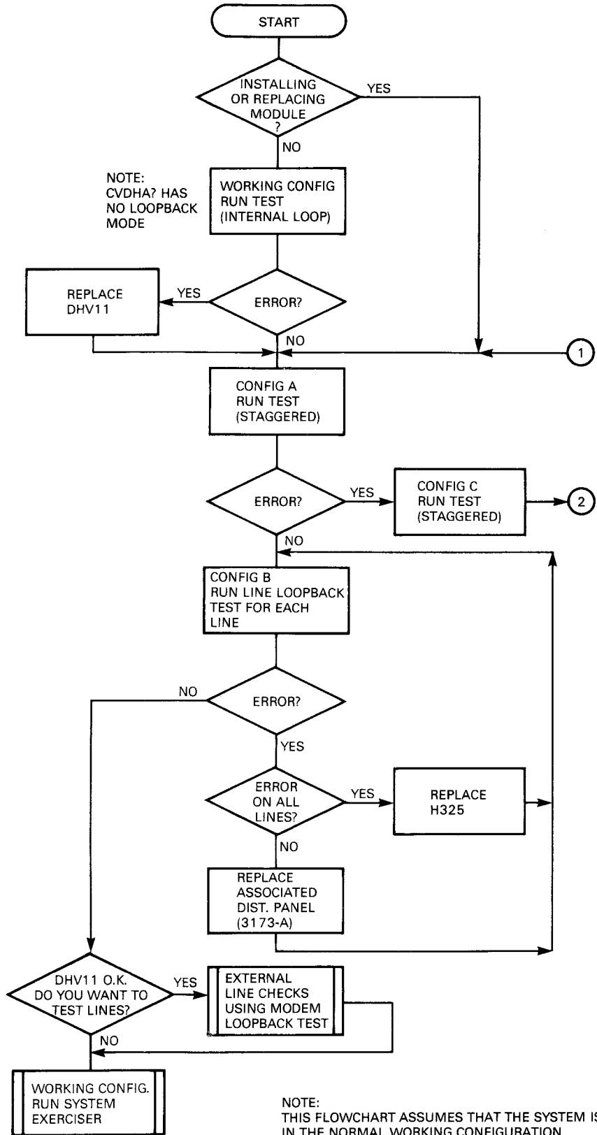
Figure 5-2 Troubleshooting Flowchart
