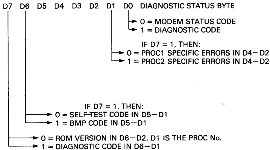
Figure 3-2 Diagnostic/Status Byte
