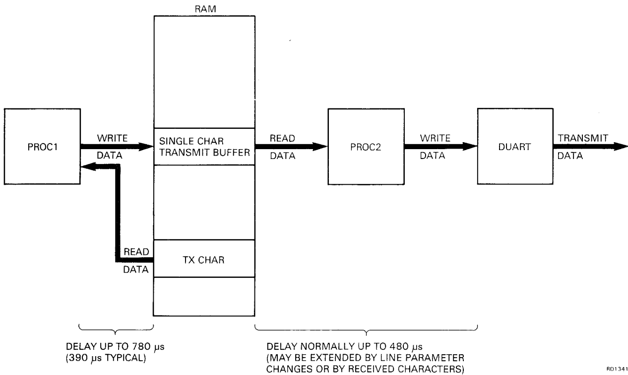
Figure 4-10 Single-Character Transmit
