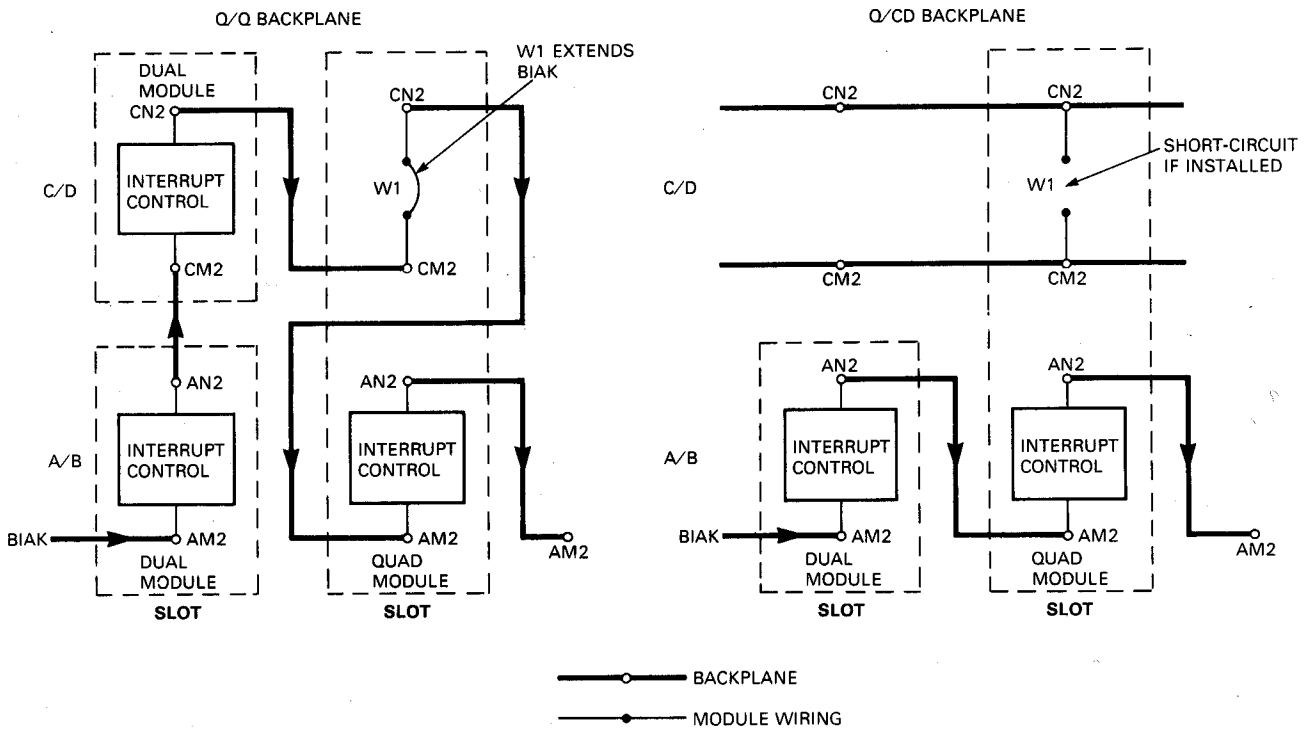
Figure 2-4 Bus Grant Continuity
