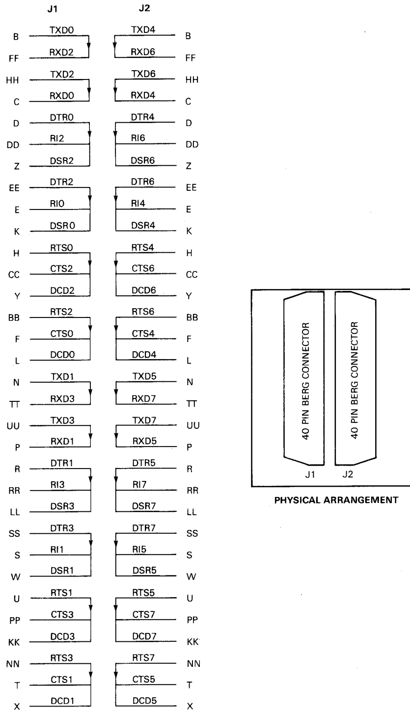
Figure 2-8 Staggered Loopback Test Connector
