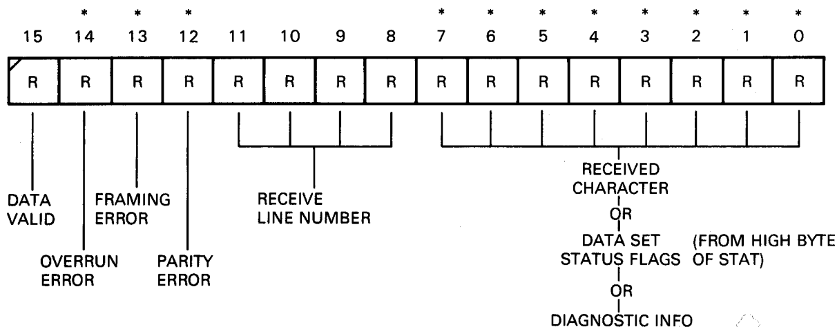
RBUF (READ BASE + 2)
