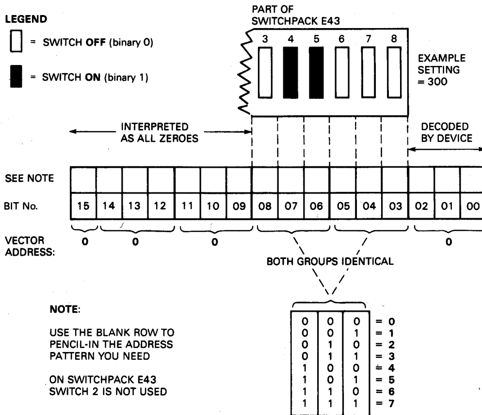
Figure 2-3 Setting the Vector Address
