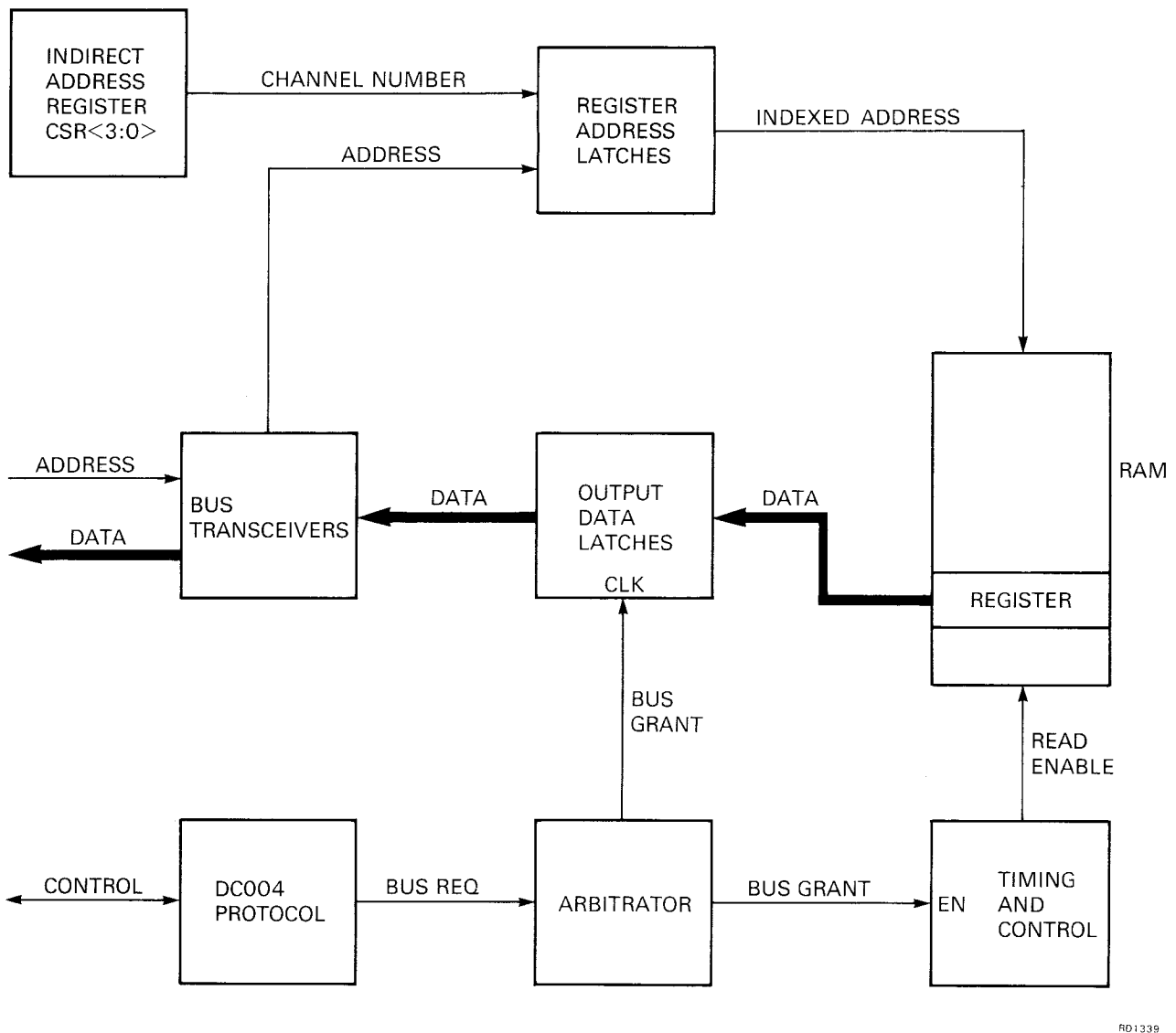
Figure 4-8 Reading from a Register
