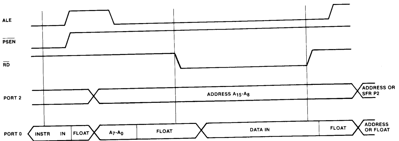
Figure A-4 Data Memory Read Cycle
