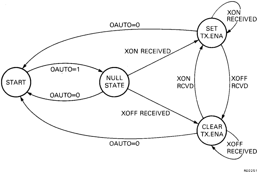
Figure D-1 Transmitted Data Flow Control
