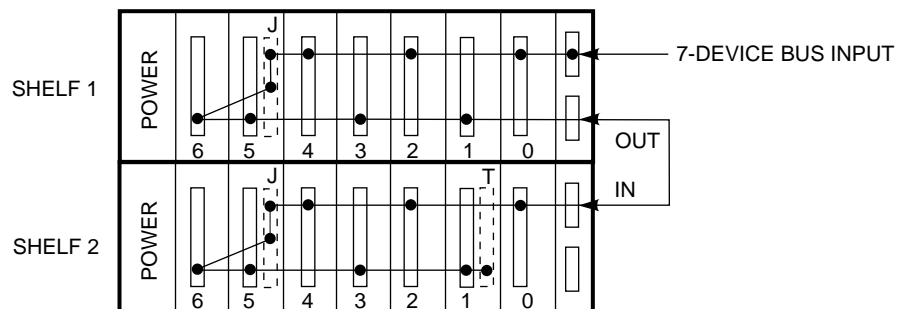
Figure 3–4 Single SCSI Bus on Two BA350–LA Shelves
