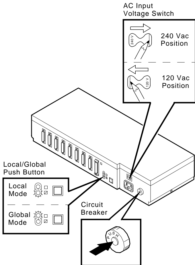
Figure 1-2 DELNI Controls and Indicators
