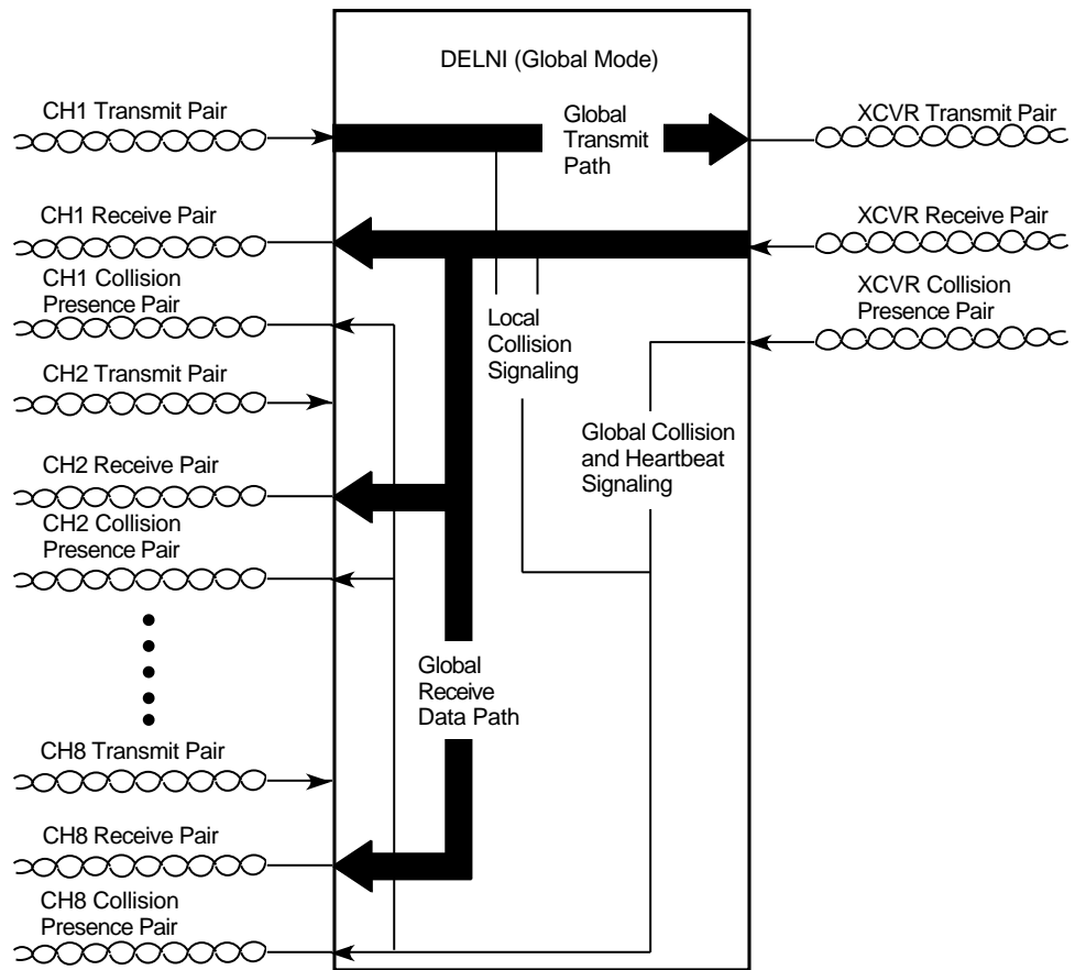
Figure 3-3 GLOBAL Mode Signal Flow Diagram
