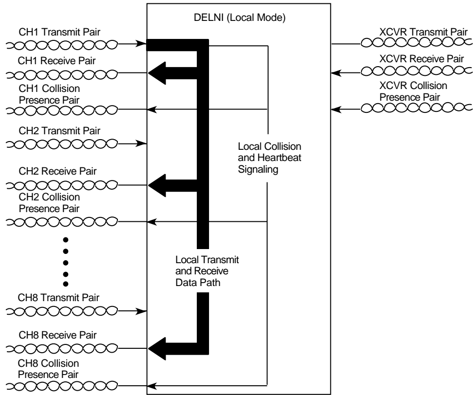
Figure 3-1 LOCAL Mode Signal Flow Diagram
