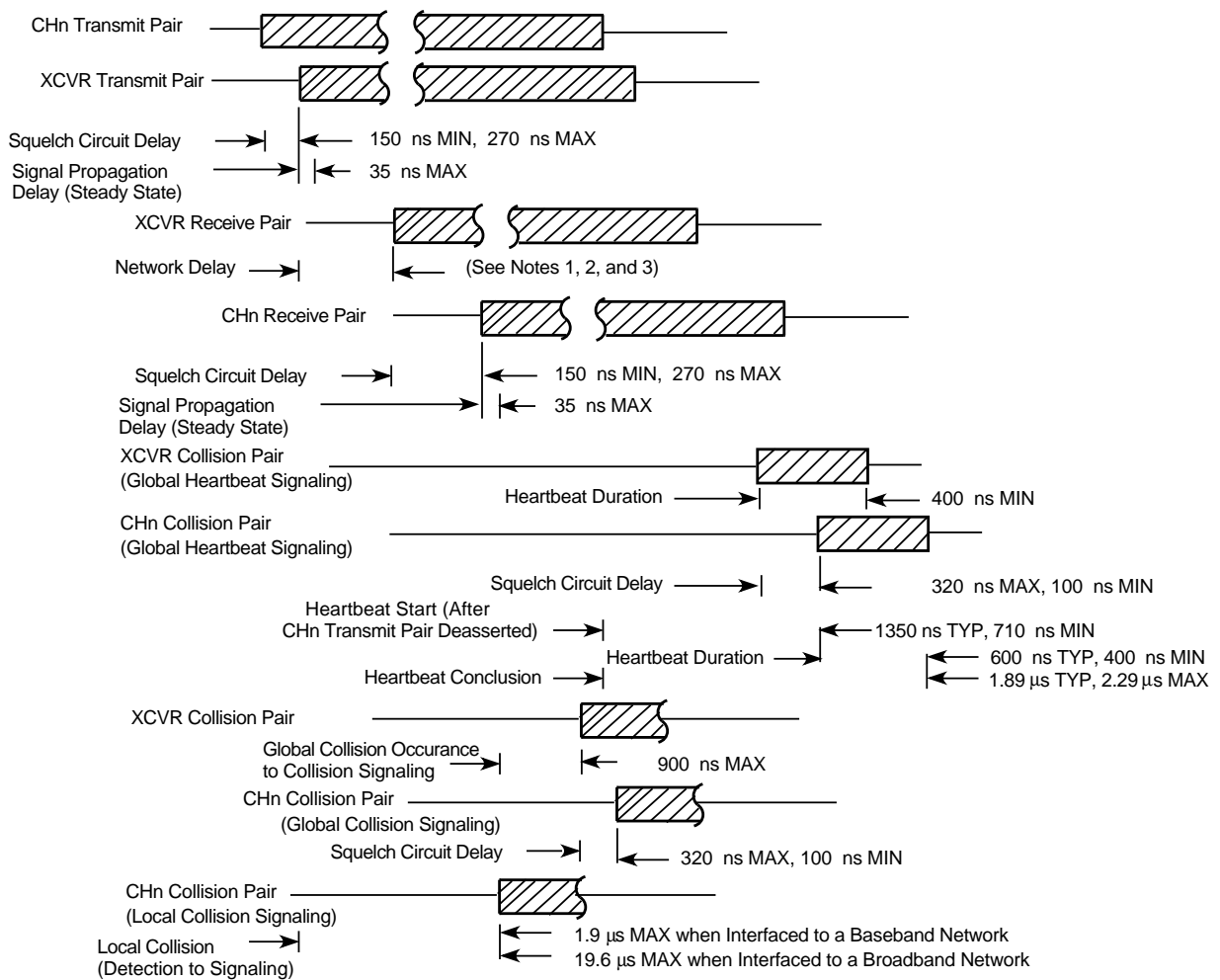
Figure 3–4 GLOBAL Mode Signal Timing Diagram
