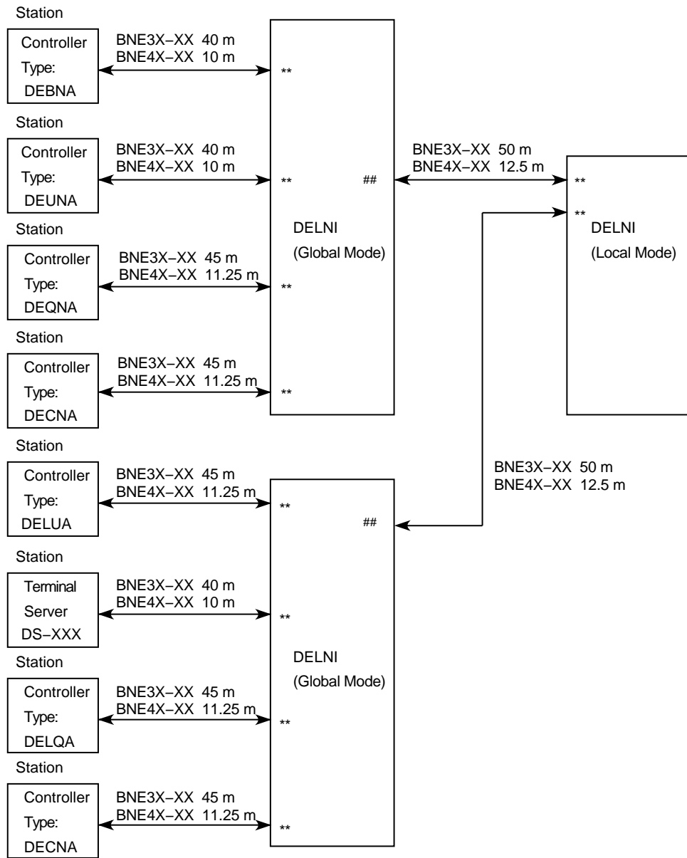
Figure 2-2 Configuration Guidelines and Limitations: Two-Tier DELNI LAN
