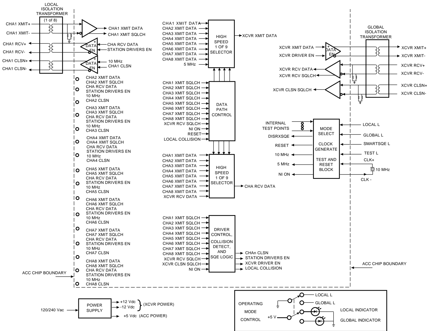
Figure 4-1 DELNI Functional Block Diagram
