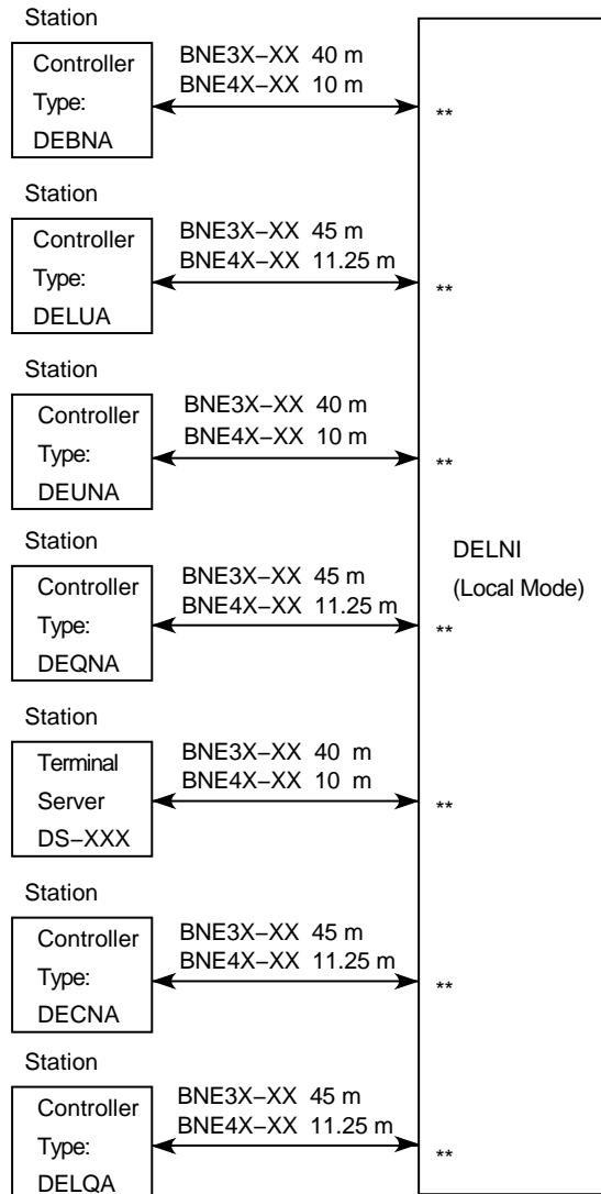
Figure 2-1 Configuration Guidelines and Limitations: Standalone DELNI LAN
