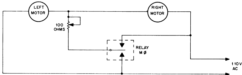
Figure 5-5 Relay M0 Function
