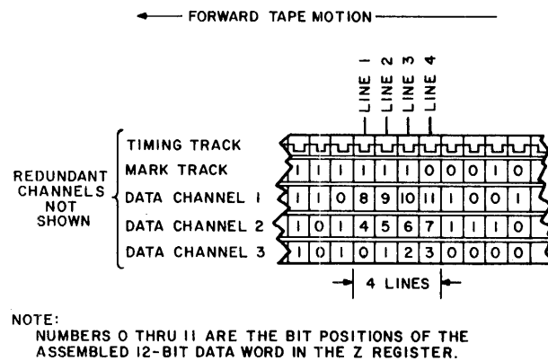
Figure 3-2 Structure of 12-Bit Data Word (4 Tape Lines)
