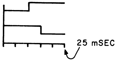
Figure 5-10 Waveform for N.O. Contacts
