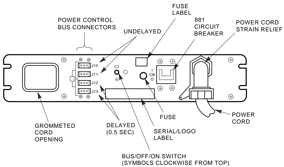
Figure 4-2 Power Controller
