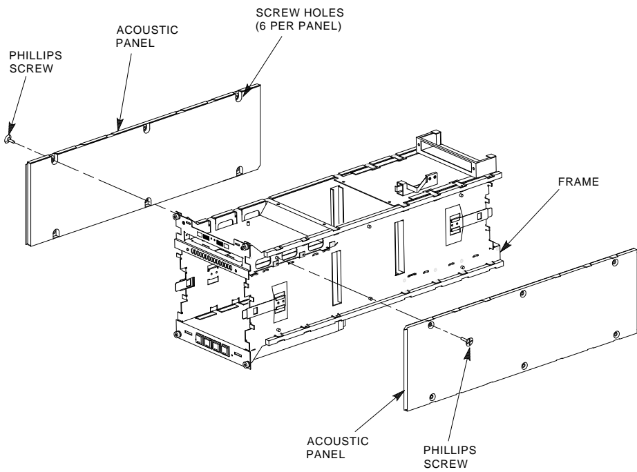
Figure 6-17 Removing the Acoustic Panels
