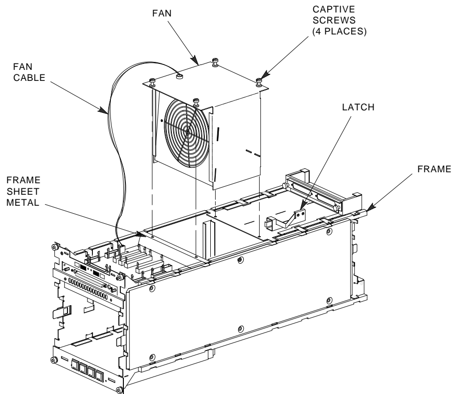
Figure 6-11 Removing and Replacing the Fan Assembly
